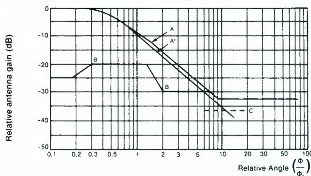
Co-polar and cross-polar reference patterns for receiving antenna in Regions 1 and 3 Curve A: Co-polar component for individual reception without sidelobe suppression Curve A': Co-polar component for community reception without sidelobe suppression Curve B: Cross-polar component for both types of reception Curve C: Minus the on-axis gain
