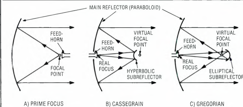
Figure 3. Symmetrical reflector antenna types.
