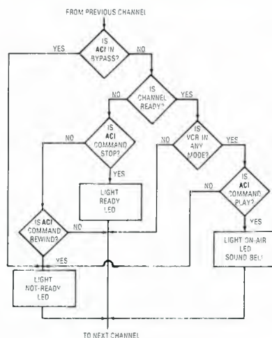
Figure 1. The flow chart for the computer program used for each channel. There are six decisions, some of which are for protection in case the operator does not follow procedures correctly. If the channel is Ready (tape cued) and the operator puts the videotape machine into any mode, a Not ready indication will result.
