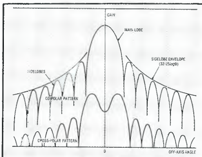
Figure 2. Typical antenna radiation patterns. An improved sidelobe envelope would decrease sidelobe levels.
