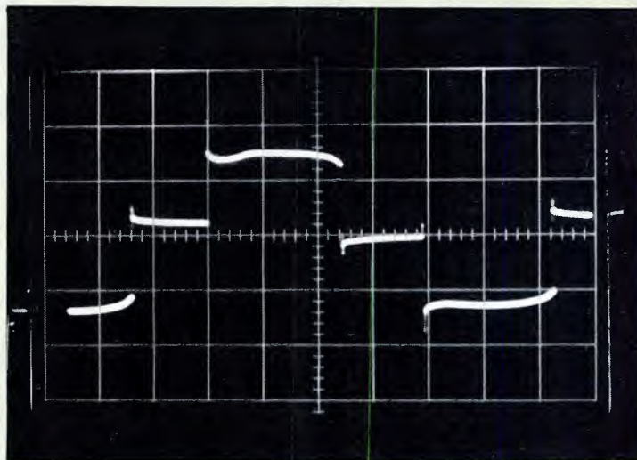
Figure 3. The stepped square-wave output of the 1409 UPS inverter.
